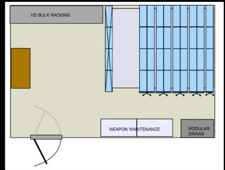
High Density Design Example – Increase Usable Floor Space or Double Storage Capacity With Additional Mobile Carriages
