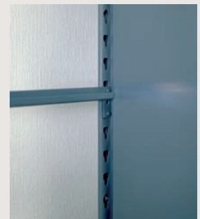
Wedge-Locking Double Rivet with Visual Index Keyholes – Exceptional strength and rigidity without sway braces or nuts and bolts.
